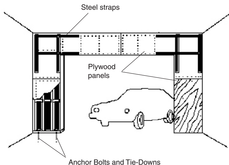
Figure 28—Bracing garage walls. If your house has a room over the garage, the garage walls may not be strong enough to hold up during an earthquake unless they are braced with plywood panels and steel straps.
